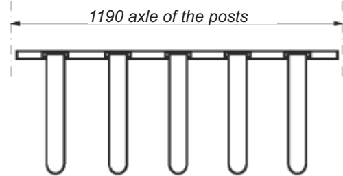
Set of tongues SW 030.015
